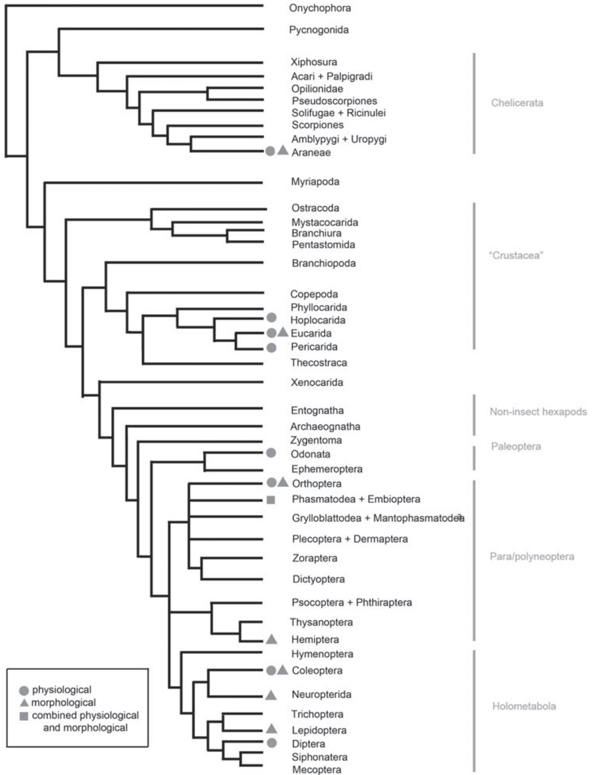
Fig. 4. Phylogenetic distribution of reversible colour change in Arthropoda. Dots indicate lineages in which reversible colour change has evolved at least once; dot colour denotes underlying mechanism (● for physiological mechanisms; ▲ for morphological; ■ for both mechanisms combined). Cladogram modified from phylogenetic hypotheses of Regier et al. (2010); Trautwein et al. (2012) and Coddington (2005).
