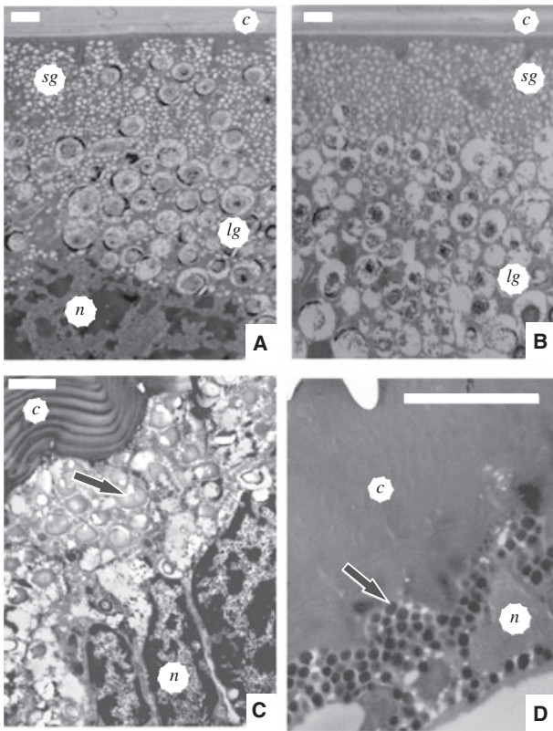
Fig. 3. Transmission electron micrographs of a cross section of the integument showing c , cuticle; sg , small granules; lg , large granules; n , nucleus. (A) Koscuscola tristis male, < 10^{\circ}\text{C} , scale bar: 1\ \mu\text{m} . (B) K. tristis male, > 25^{\circ}\text{C} , scale bar: 1\ \mu\text{m} . (C) Misumena vatia in the white phase with Type I granules (arrow), scale bar: 2\ \mu\text{m} (adapted with permission from the Journal of Experimental Biology ). (D) M. vatia in the yellow phase with Type III granules (arrow), scale bar: 10\ \mu\text{m} (adapted with permission from the Journal of Experimental Biology ).
